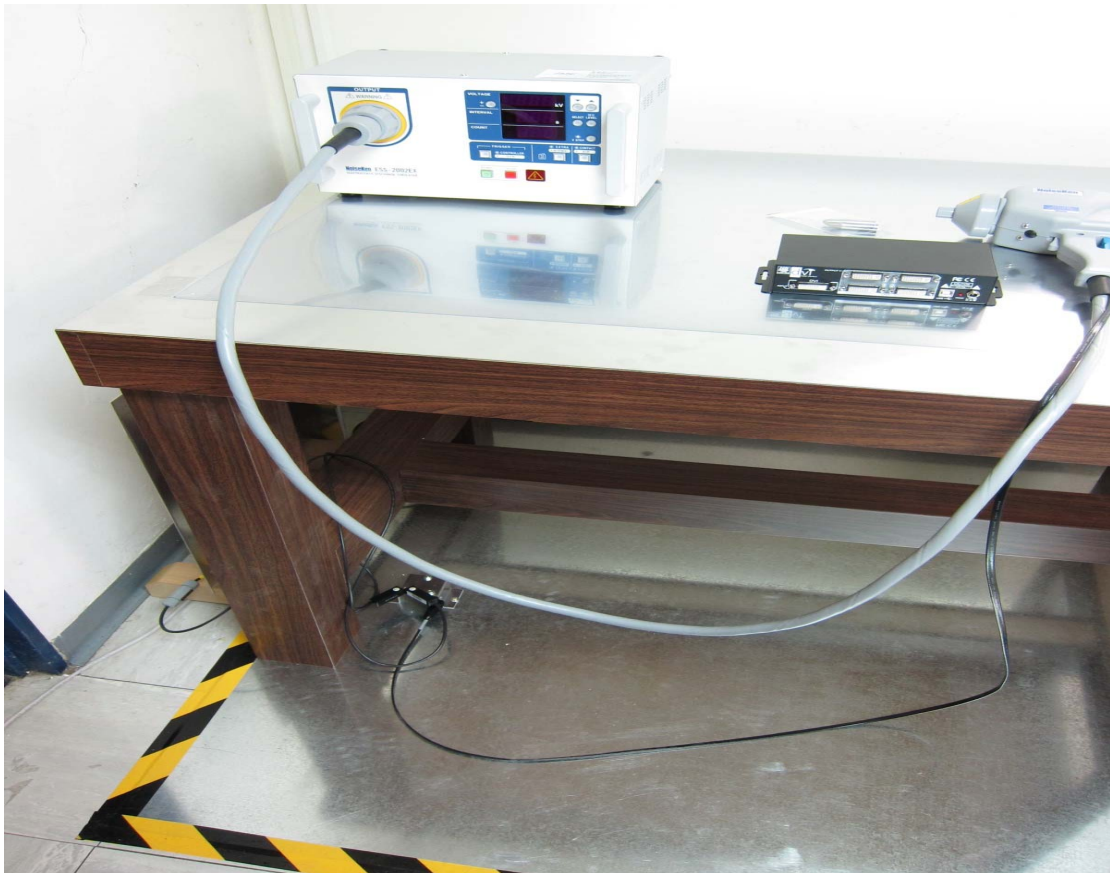
Picture 4: Adjust the voltage, interval and count for ESD testing
