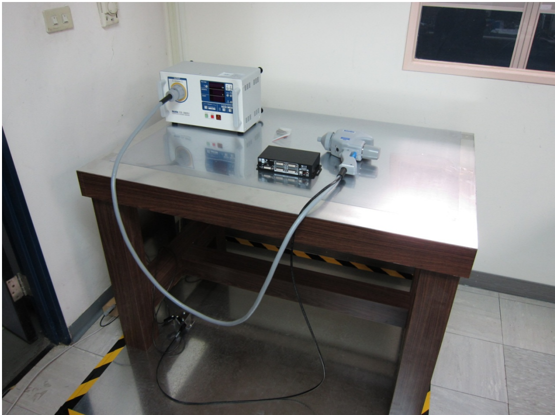
Picture 2: Discharge Gun and testing unit
